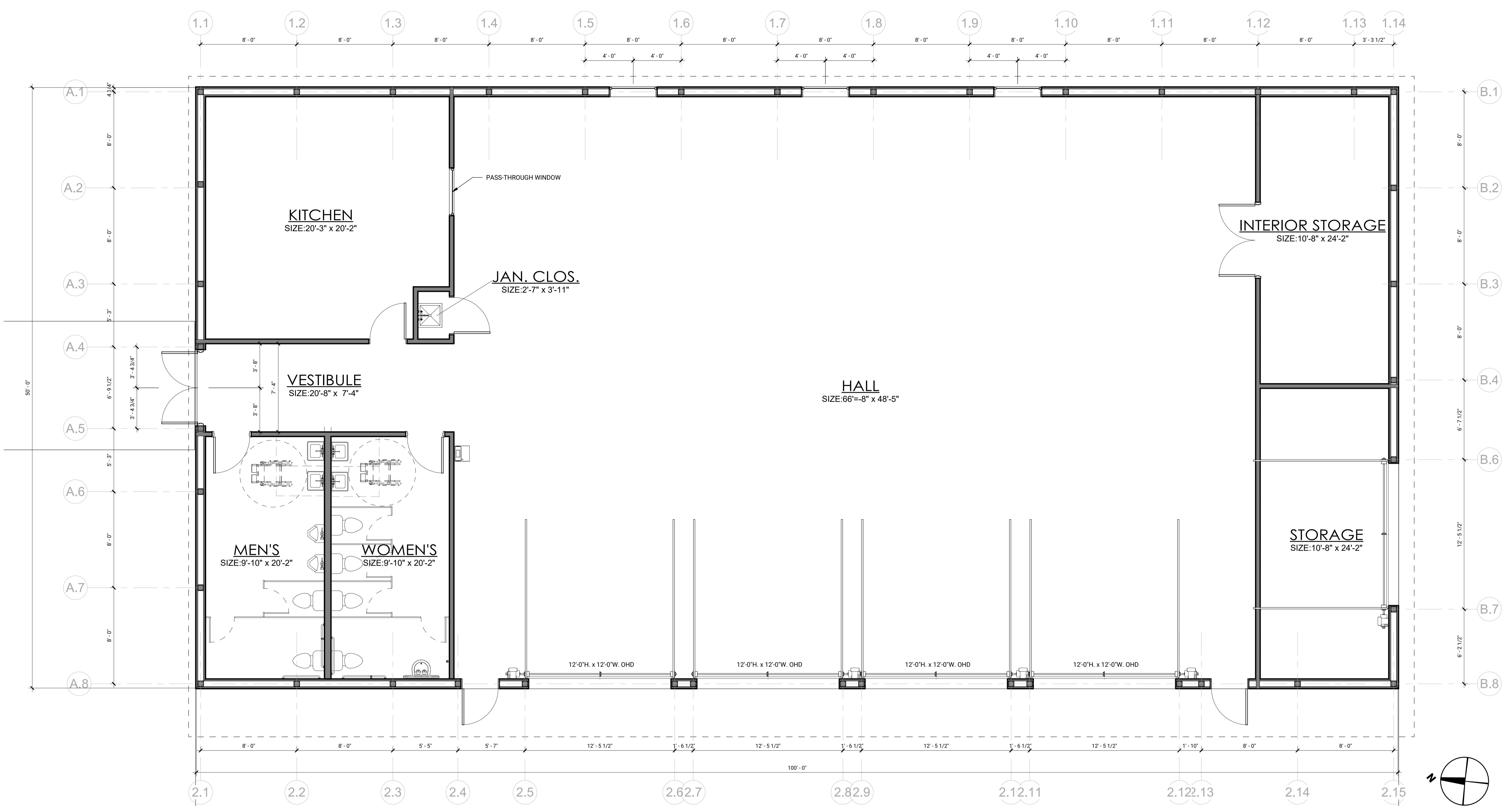
1 FLOOR PLAN A-1.10 1/4" = 1'-0"
